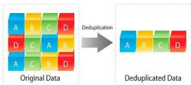
Fig 3:- Data Deduplication
