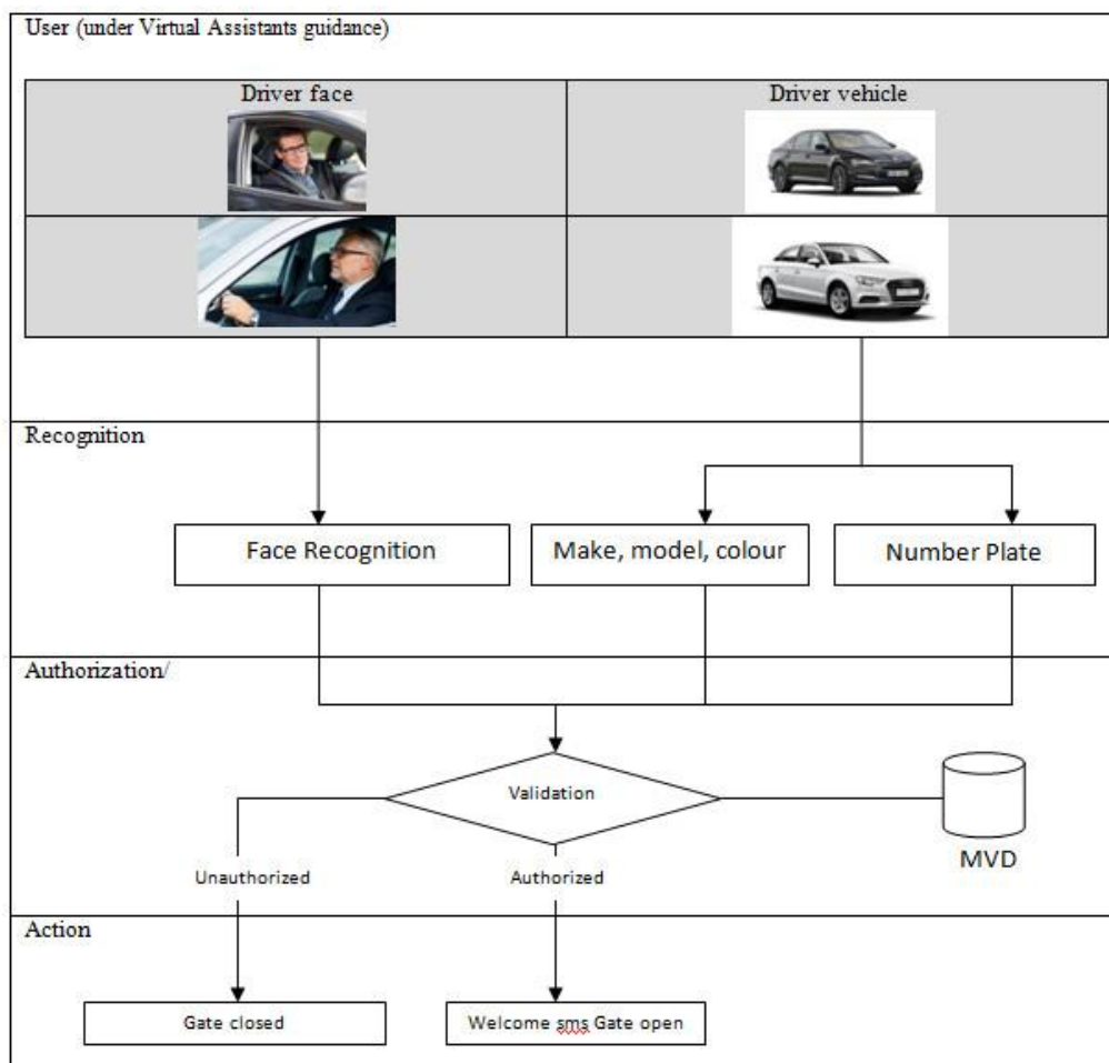
Fig 5:- System Architecture of IGNS security system
