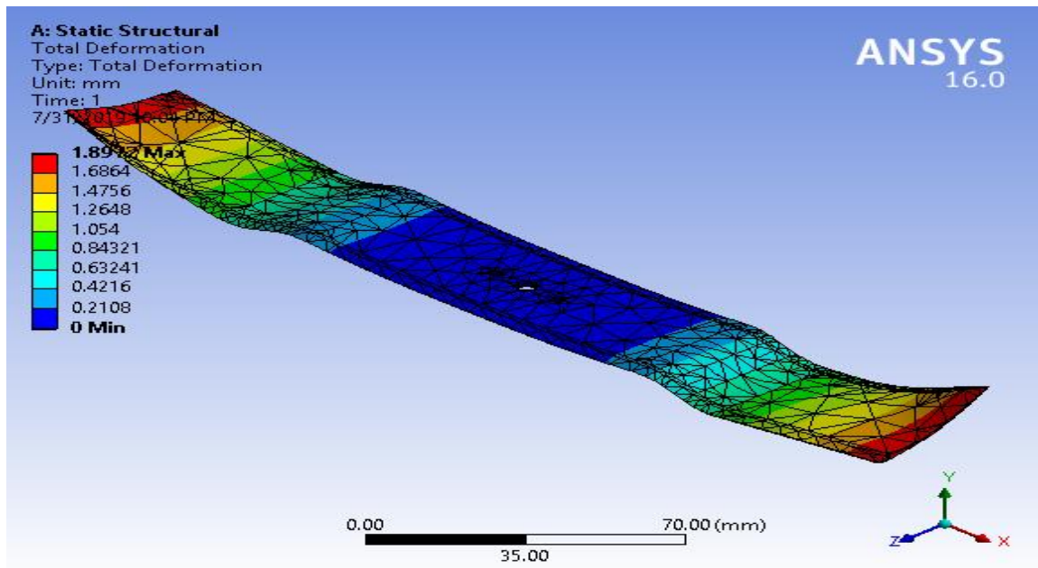
Fig 3.14: Blade model showing the total deformation
