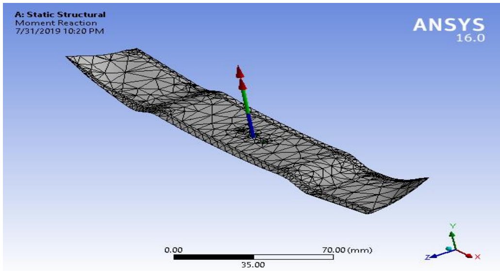
Fig 3.16: Blade model showing the bending moment of the blade
