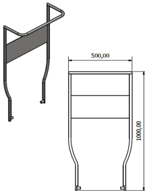
Fig 3.12: Lawn mower handle frame
