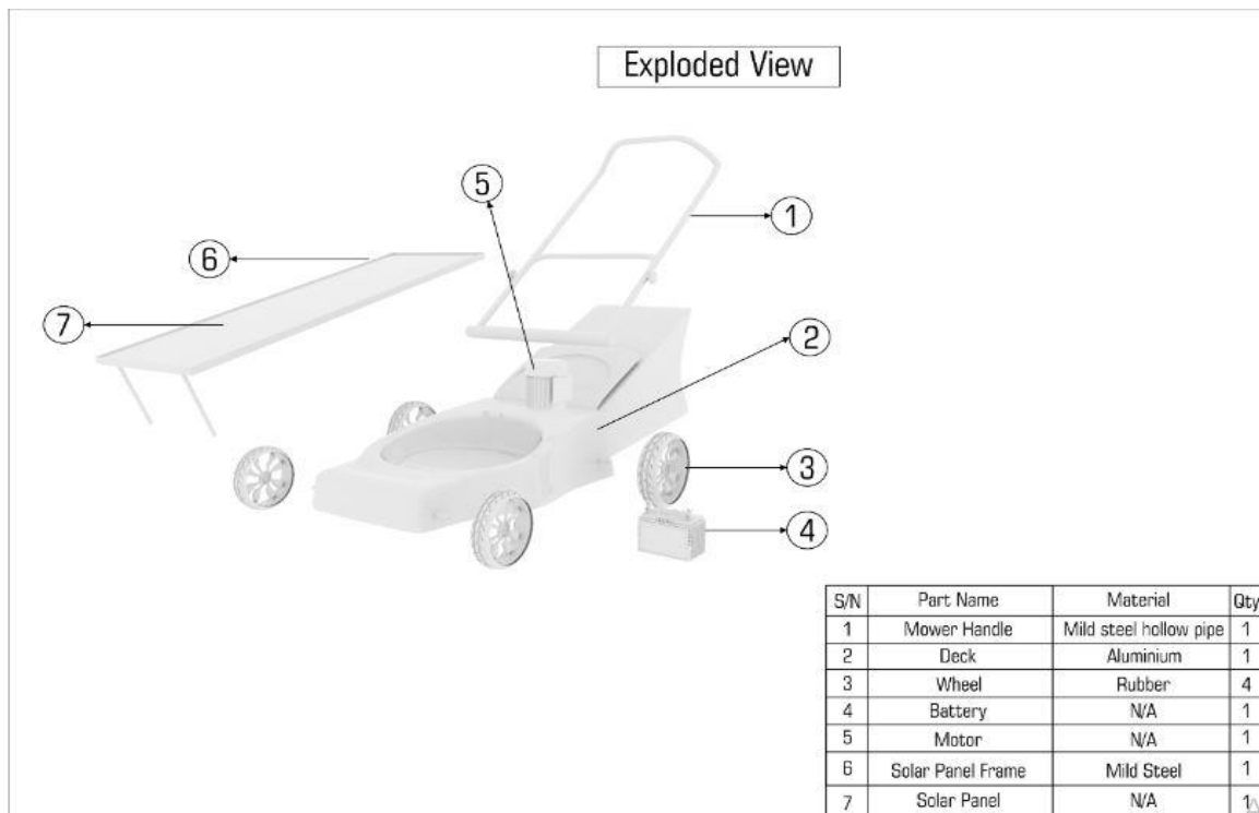
Fig 3.2:Exploded view of the proposed solar lawn mower
