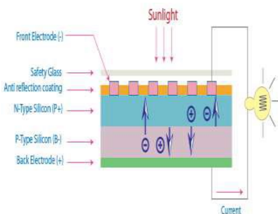
Fig 3.7: Photovoltaic principle
