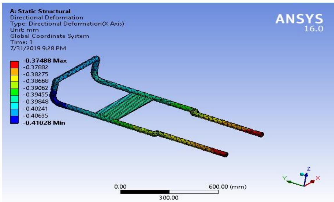
Fig 3.17: Frame model showing the directional deformation
