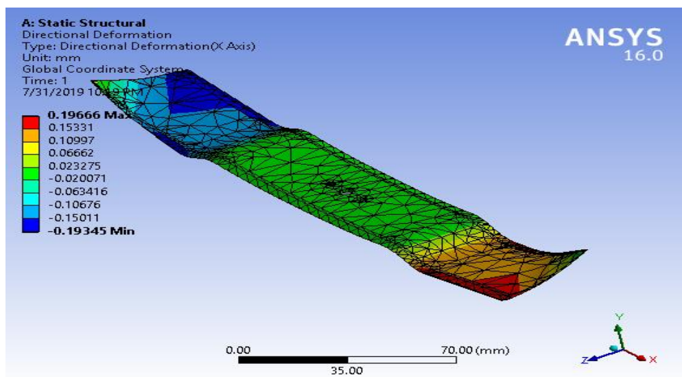
Fig 3.15: Blade model showing the directional deformation
