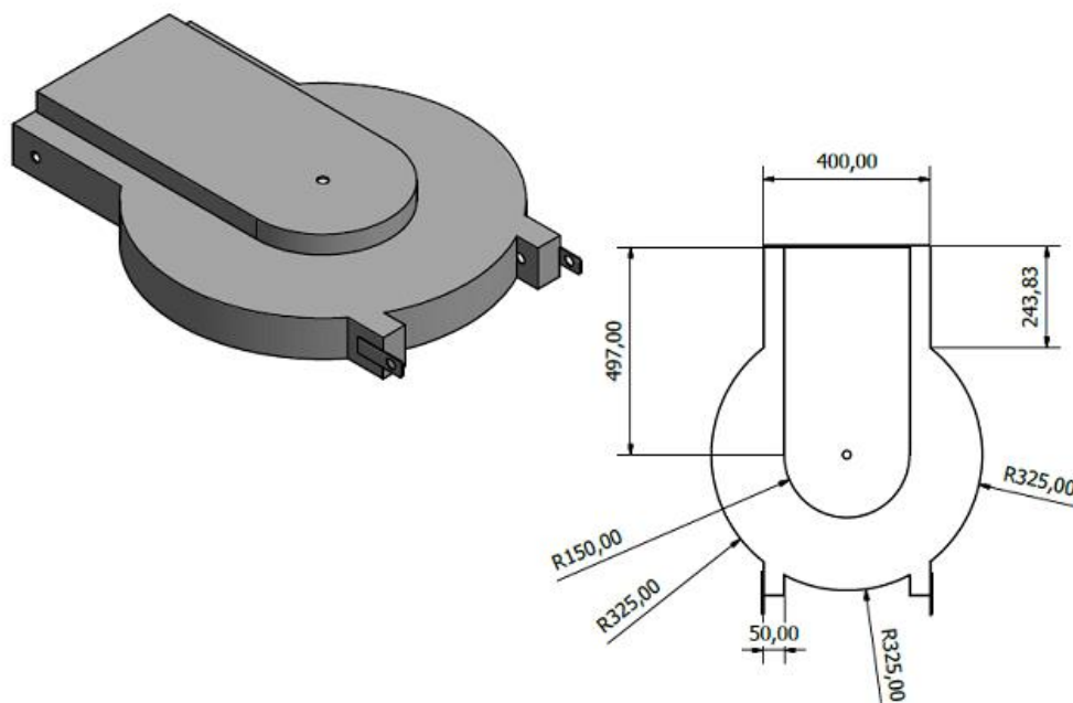
Fig 3.11: Lawn mower deck
