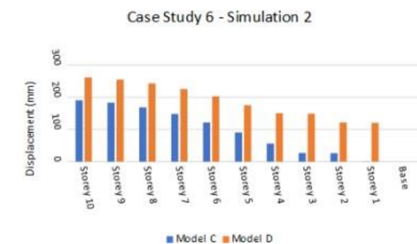
Figure 23: Graph of Maximum Storey Displacement in Case Study 6
