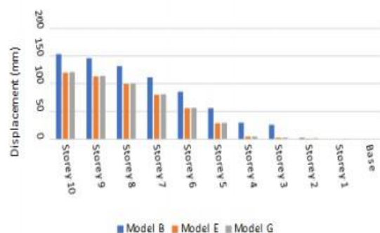
Figure 25: Graph of Maximum Storey Displacement in Case Study 6
