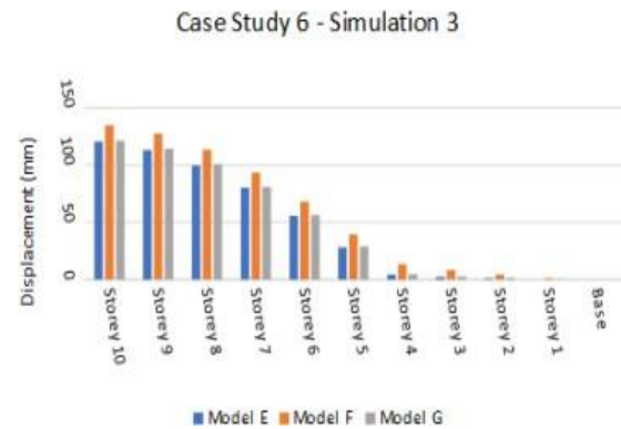
Figure 24: Graph of Maximum Storey Displacement in Case Study 6
