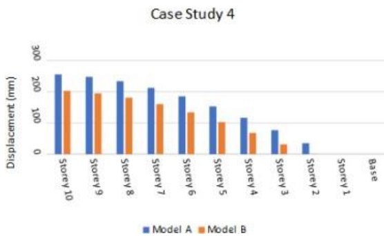
Figure 20: Graph of Maximum Storey Displacement in Case Study 4
