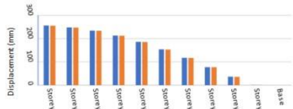
Figure 18: Graph of Maximum Storey Displacement in Case Study 2
